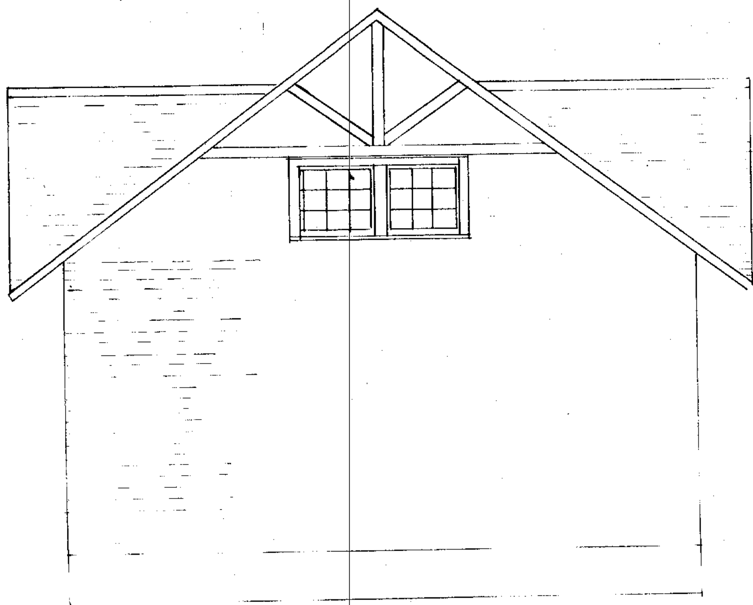
ELEVATION OF BOAT HOUSE FOR THOMAS, S.W. 1/4 SCALE 1/4"
